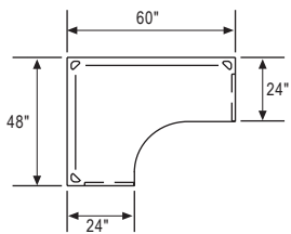
Plan view (BC24486024GF)
