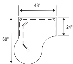
Plan View (BVPD604824G)
