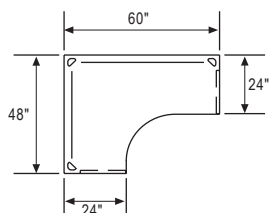
Plan view (BC24486024GP)
