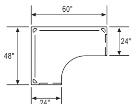
Plan view (BC24486024FF)
