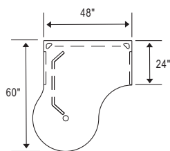
Plan View (BVPD604824P)
