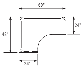
Plan view (BC24486024GG)
