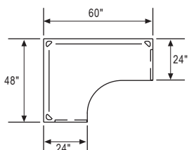
Plan view (BC24486024FG)
