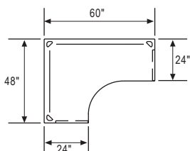
Plan view (BC24486024FP)
