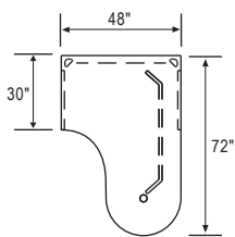
Plan View (BVP304872G)
